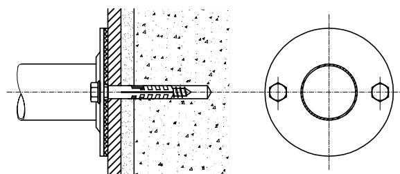
DETALLE A E= 1:2.5
