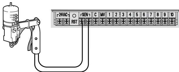
Mini-Click Rain Sensor
